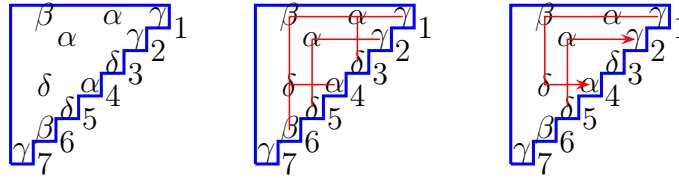
FIGURE 3. A staircase tableau, its diagram and the paths of 1 and 5
