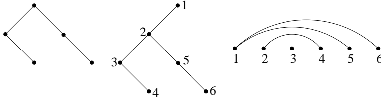
Figure 8: The bijection for Exercise 6.19(d 5 )
