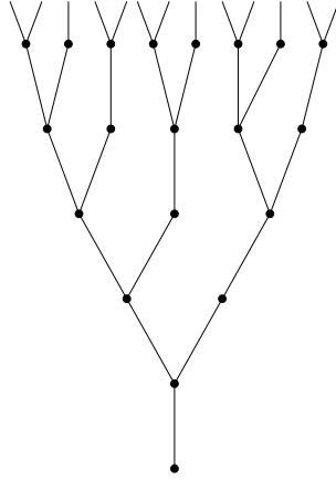
Figure 5: The Fibonacci tree
