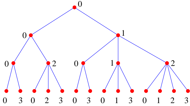
Figure 9: The tree for Exercise 6.19(u 5 )
