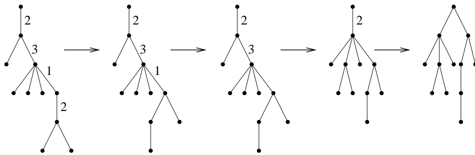
Figure 7: An example of the bijection of item (uuu)
