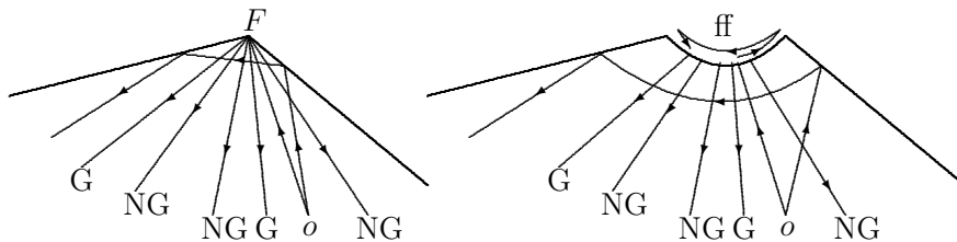
FIGURE 2. Geometric optic rays hitting a corner F , emanating from a point o . The rays labelled G are geometric at F , while those labelled NG are non-geometric at F . The leftmost geometric ray is a limit of rays like the unlabelled one shown on the figure that just miss F . The blown up version of the picture, i.e. where (r, \theta) are introduced as coordinates at the origin, is shown on the right. The front face (i.e., the lift of the corner) is denoted ff . The reflecting line indicates the broken geodesic of length \pi induced on ff given by r = 0 , \theta \in [0, \theta_0] . The total length of the three segments shown on ff is \pi ; this can be thought of as the sum of three angles on the picture on the left: namely the angles between the incident ray and the right boundary (corresponding to the first segment), the right and left boundaries, finally the left boundary and the emanating reflected ray.
