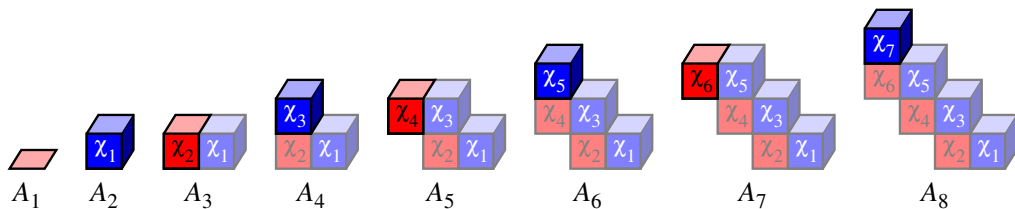
FIGURE 2. The bi-diagonal models for the positive eigenvalues of the anti-GUE form a one-parameter family, where each is obtained from the previous by adding a single non-zero matrix element.
