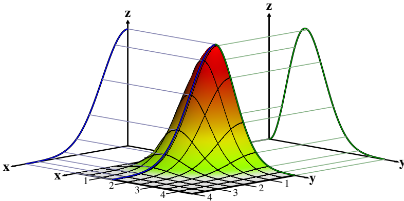
FIGURE 9. The function g(x, y) = \frac{e}{2}y^2e^{-x^2/2-y^2/2} is separable with a maximum value of g(0, \sqrt{2}) = 1 and satisfies the relation g(x, y) = g(x, \sqrt{2}) \times g(0, y) . The factors correspond to the fact that the singular values of the 2 \times 2 GUE have the same distribution as independently distributed \chi_1 and \chi_3 random variables.
