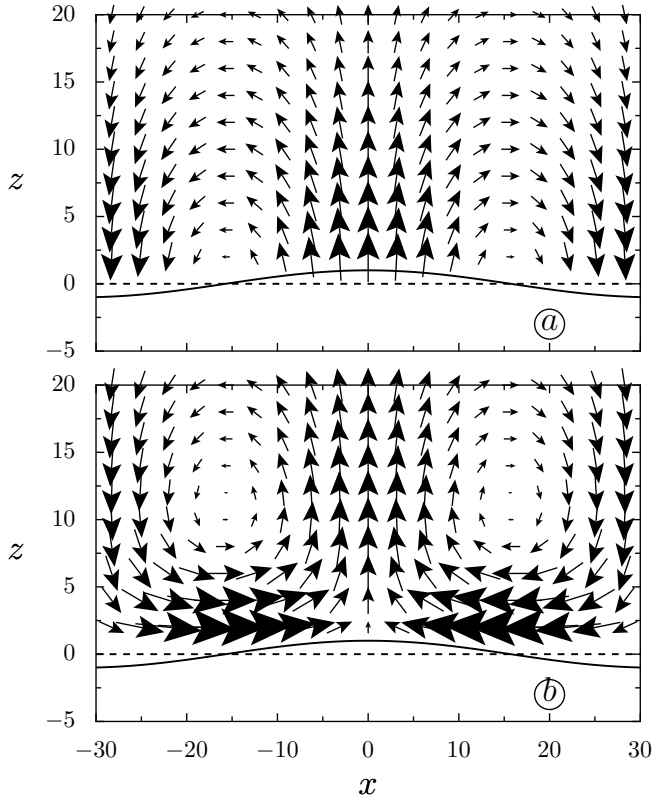
Fig. 4. Two types of fluid flow around a perturbed, driven membrane. (a) The membrane bending mode with associated flow field [47], in the absence of any applied electric field: \sigma = 0 . In this case, it is the motion of the membrane which drives the flow field by the incompressibility condition. For a growing sinusoidal perturbation, streamlines connect the peaks to the valleys. The membrane seen edge-on as a solid line, undergoes a bending wave of wavevector 0.1 (or of wavelength 20\pi ) and of amplitude 0.1. Note that the height of the membrane has been multiplied by an extra factor 10 for improved visualization. The undeformed membrane is shown edge-on as a dashed line. (b) Vortices of induced-charge electro-osmosis (ICEO) for a non-moving curved membrane, due to effective slip from the valleys to the peaks, as explained below. Unlike the case (a), here it is the flow field induced by ICEO which determines the modulation of this non-moving membrane. An applied field is applied which corresponds to \sigma = 30 . In this example, as in biological membranes, the double layers are thin compared to the wavelength of the perturbation k_{\perp} = k_{\perp}^*/\kappa \ll 1 . The calculation also assumes linear response to a small amplitude perturbation, \kappa h^* \ll 1 . In these figures, this condition is satisfied since h = 0.1 , and the unit length corresponds to one Debye length.
