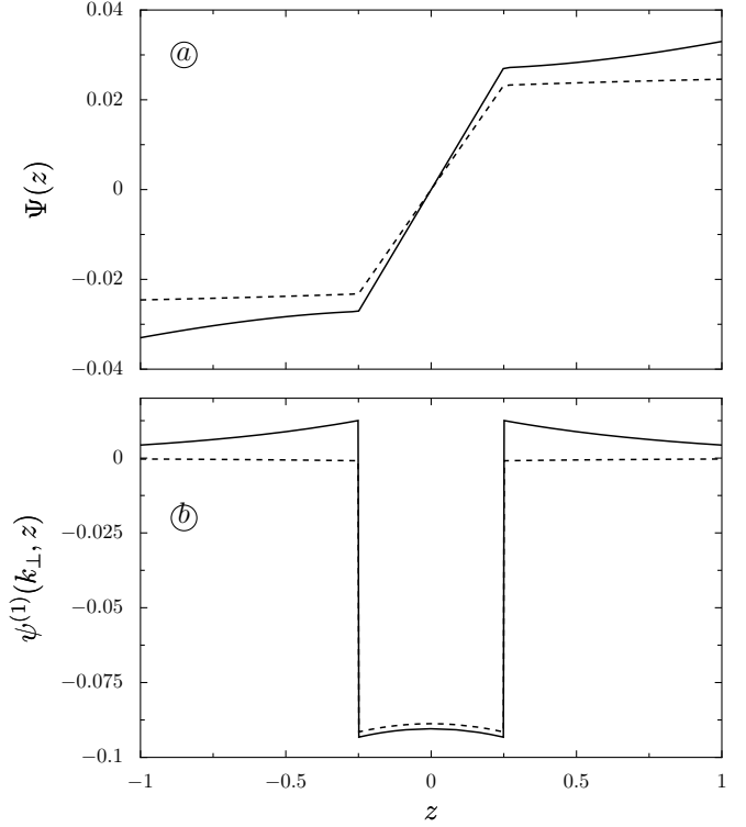
Fig. 7. Solutions of the electrokinetic equations for a membrane of finite thickness and symmetric ions concentrations. The electrostatic potential \Psi(z) is shown in (a) and the first order correction to the potential \psi^{(1)}(\mathbf{k}_\perp, z) is shown in (b). We use dimensionless units and the following parameter values L = 100 , V = 2 , G_1 = G_2 = 1 , d = 0.5 , r = 1/40 and k_\perp = 1 for the solid line, and the same parameters except for G_1 = G_2 = 0.01 and V = 0.1 for the dashed line. The difference between the solid line and the dashed line is that the solid line corresponds to a situation with a negative value of \tilde{\sigma} with an upward slope of the potential near z = d/2 , while the dashed line corresponds to a situation with a positive value of \tilde{\sigma} with a downward slope of the potential near z = d/2 .
