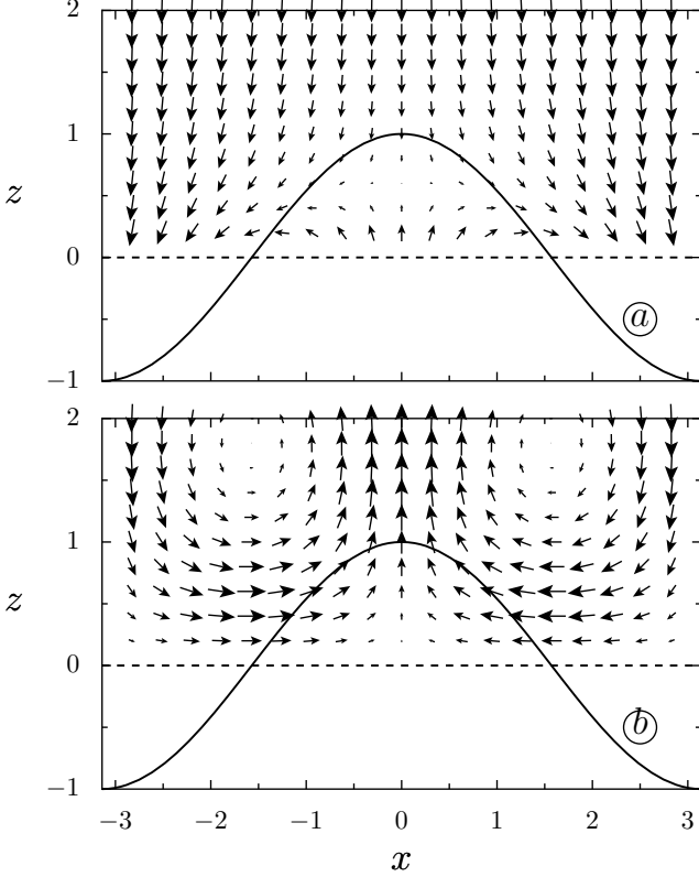
Fig. 6. Induced-charge electro-osmotic (ICEO) flow around a driven membrane in the regime of thick double layers k_{\perp} = k_{\perp}^*/\kappa^* \approx 1 , where the thickness of the Debye layer is comparable to the wavelength of the shape perturbation and to the amplitude of modulation of the membrane. Indeed in units of the Debye layer, the amplitude of modulation of the membrane is 1, the wavevector is also 1 and the applied field corresponds to \sigma = 8 . (a) The total electric field \mathbf{E} avoids the protrusion peak due to the large positive bound charge on the membrane, even though the (much smaller) induced charge in the diffuse layer is negative at the peak and positive in the valley. (b) Vortices of induced-charge electro-osmotic flow, scaling as E^2 , and driven from the valleys to the peaks by tangential fluid forces as in the thin double layer case of Fig. 4, but with stronger effects of normal forces in the recirculating regions, as explained in the text.
