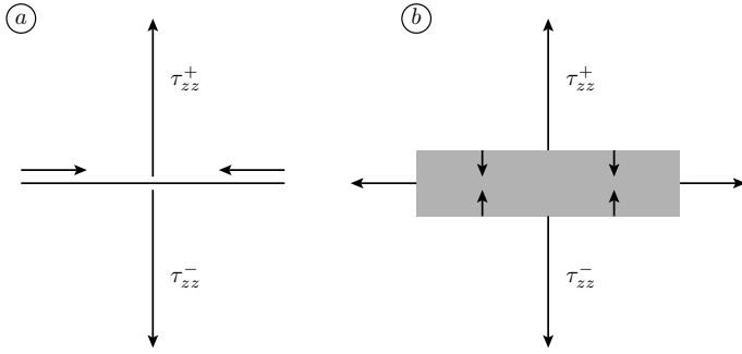
Fig. 2. Electrostatic corrections to the membrane tension for a membrane of zero thickness (a) and finite thickness (b). The Maxwell stresses are represented by vertical arrows while the horizontal arrows represent the resulting tension on the membrane as a consequence of incompressibility.
