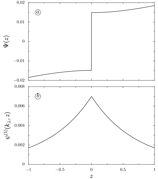
Fig. 3. Solutions of the electrokinetic equations for a membrane of zero thickness and symmetric ion concentrations. The electrostatic potential \Psi(z) is shown in (a) and the first order correction to the potential \psi^{(1)}(\mathbf{k}_\perp, z) is shown in (b). We use dimensionless units and the following parameter values V = 1 , L = 100 , G_1 = G_2 = 1 and k_\perp = 1 . In these conditions, \sigma = 0.01 .
