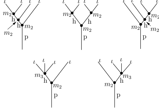
FIGURE 1. The full collection of rooted trees with 4 inputs specifying the multiplication m_4 described by Proposition 2.3.
