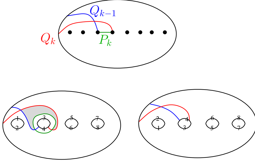
FIGURE 7. The top row above shows curves p_k , q_{k-1} , and q_k in the disk D_m , while the bottom row shows their lifts to Lagrangians in the double branched cover \Sigma (the figures on the left and right are identified according to the numbers). The shaded triangle gives rise to a non-trivial multiplication map m_{(1|1|0)} : \text{Hom}(Q_k^\Sigma, Q_{k-1}^\Sigma) \otimes \text{Hom}(Q_{k-1}^\Sigma, P_k^\Sigma) \rightarrow \text{Hom}(Q_k^\Sigma, P_k^\Sigma) .
