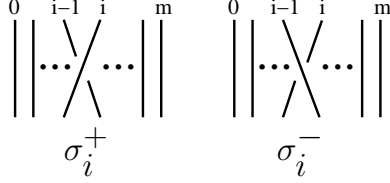
FIGURE 4. The elementary Artin generators, \sigma_i^\pm
